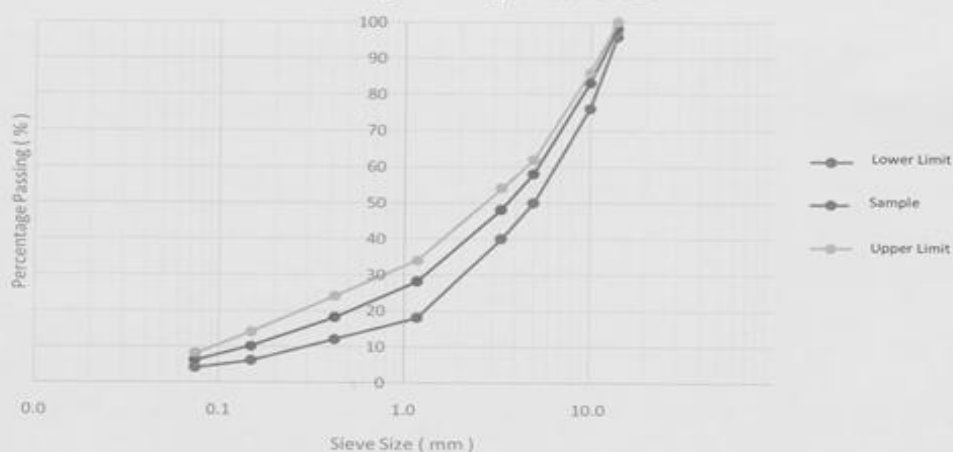
Percentage Passing vs Sieve Size
